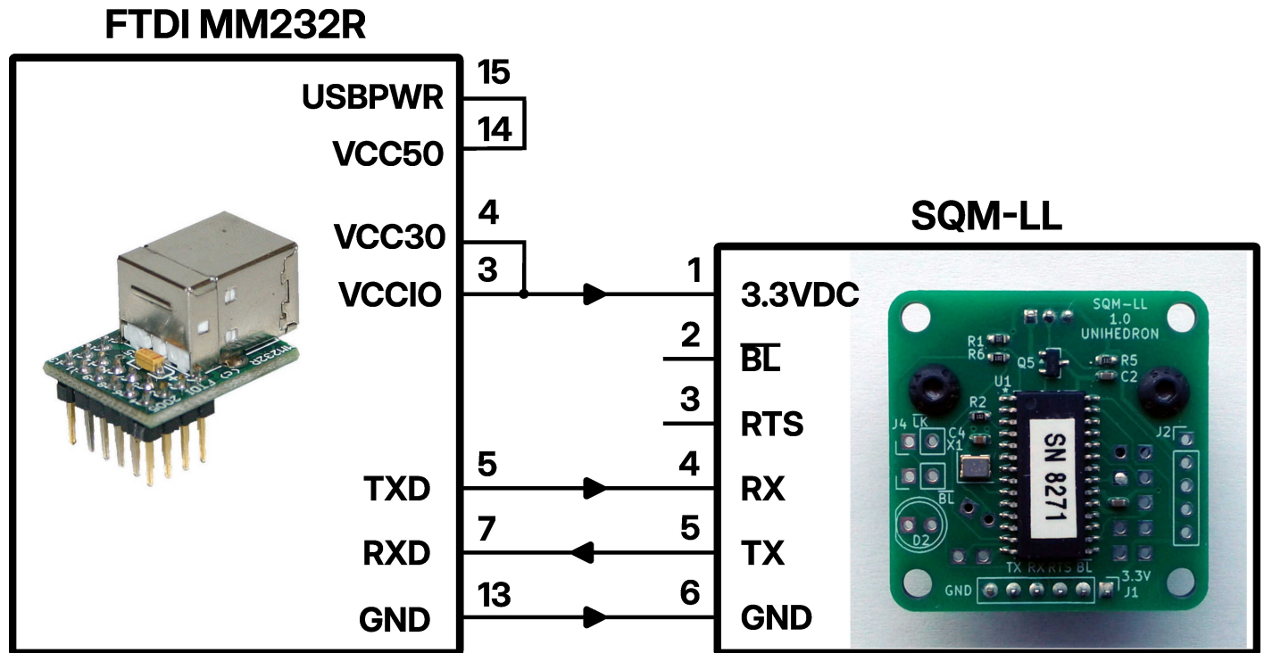
Figure 5.2: SQM-LL test setup
